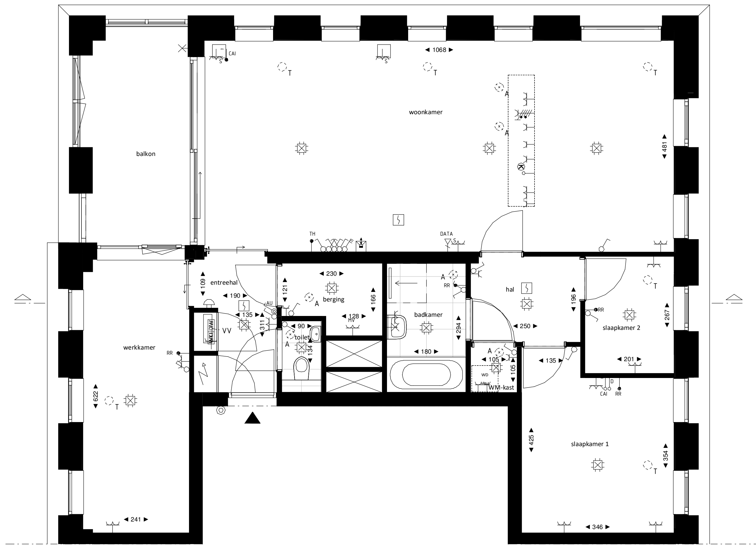
Regular 1:50
