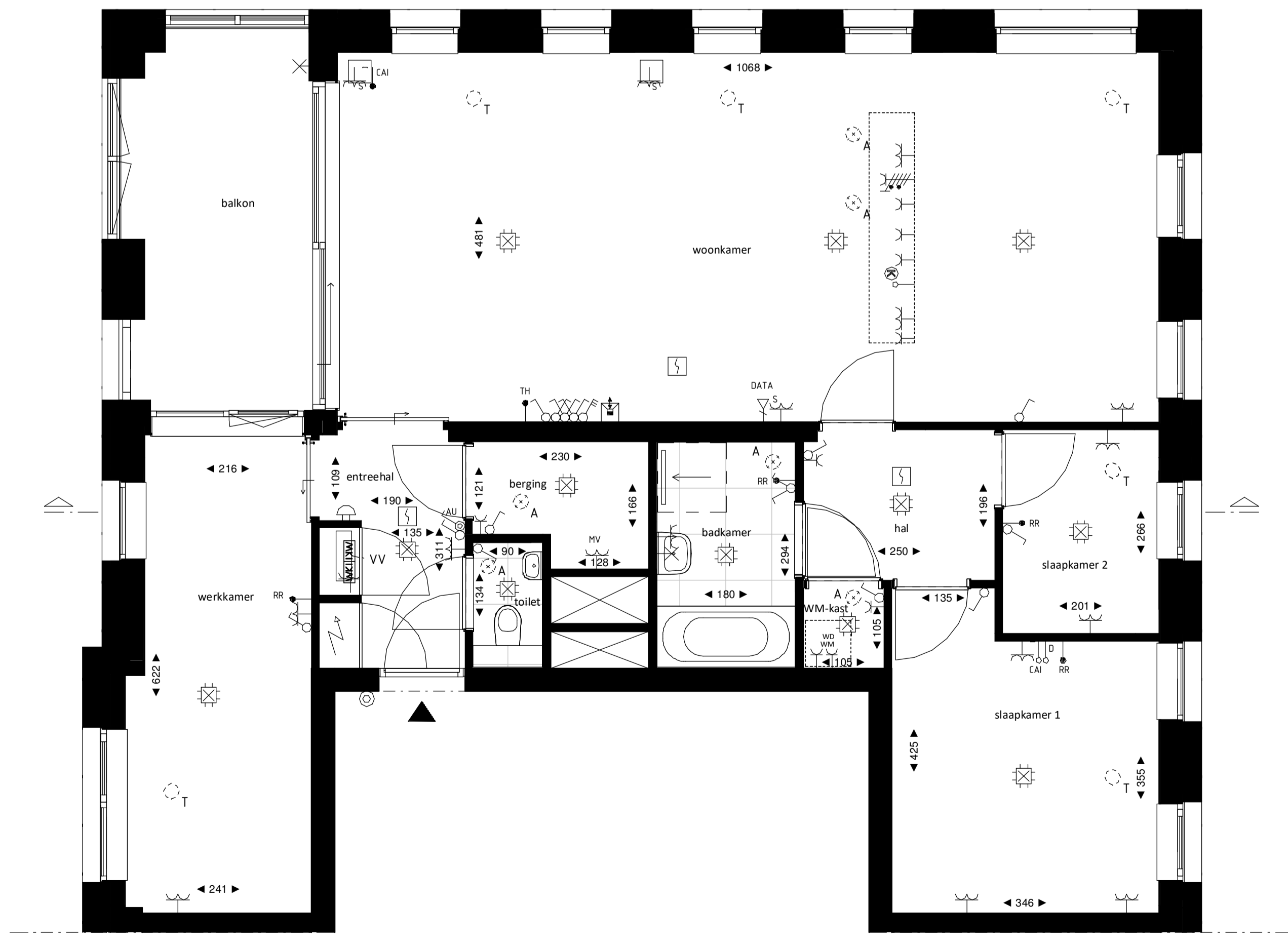
Regulier 1:50
