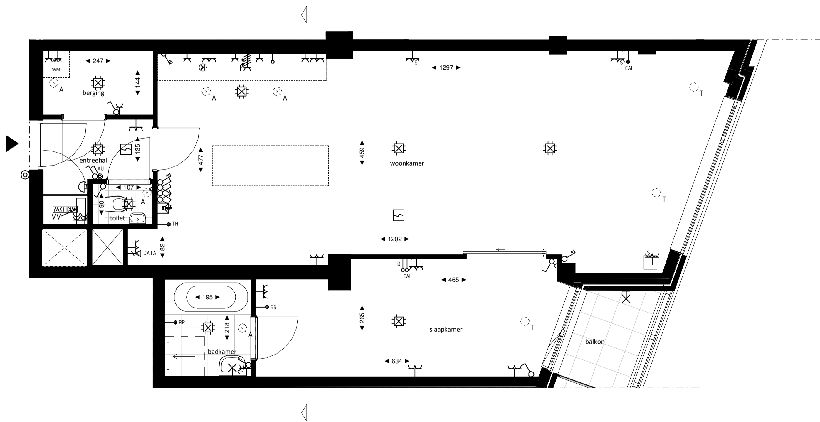
Regular 1 : 50
